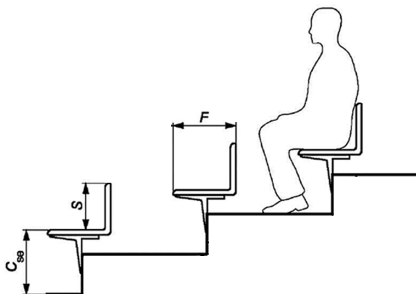
Diagram 19 Spectator seating recommendations
